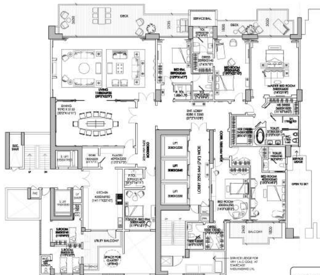
TYPICAL 5 BEDROOM UNIT OF S+38 STOREY BUILDING ( WITH 3 MAIN LIFTS )
